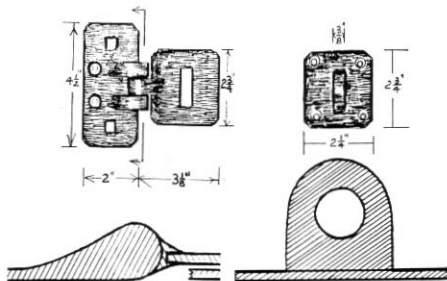
Detail of Hasp at Knuckle FULL SCALE Detail of Staple FULL SCALE
